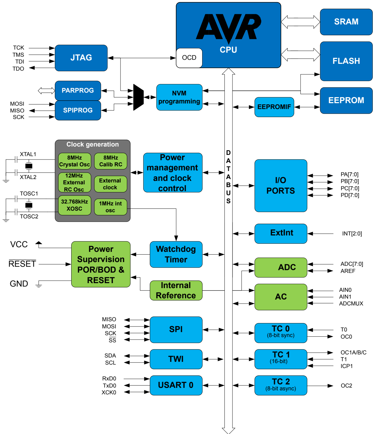
Figure 4-1 Block Diagram
