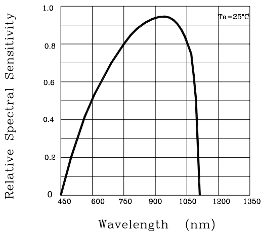
Fig. 5 Spectral Sensitivity
